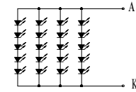
LED电路图 (5串*4并=20LED)
