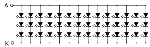
Circuit Diagram(LED:3*14=42 Dies)
